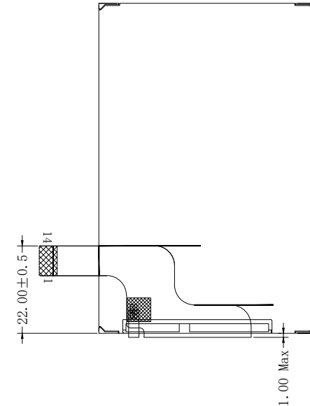
Bending diagram
